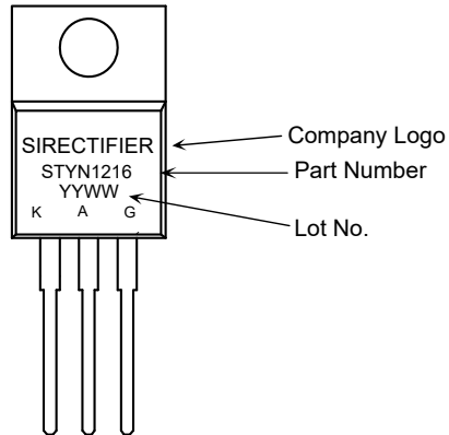
STYN1216 (TO-220AB)
