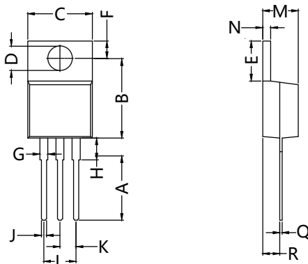
Dimensions TO-220AB
